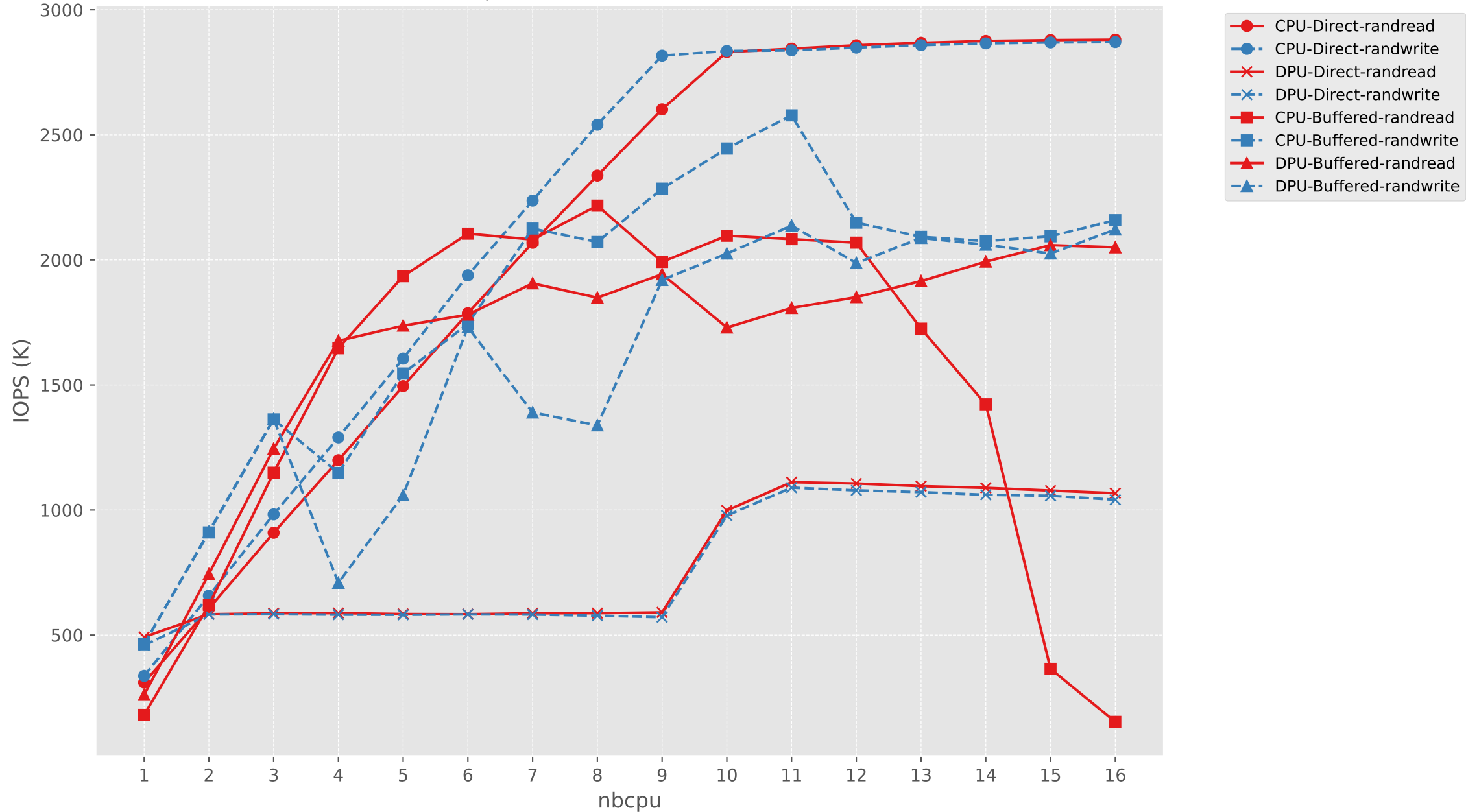
IOPS vs nbcpu (CPU vs DPU, Direct vs Buffered)
